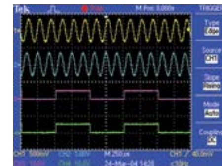
Make floating and differential measurements, accurately and quickly with four Isolated Channel inputs and isolated external trigger 3 .
