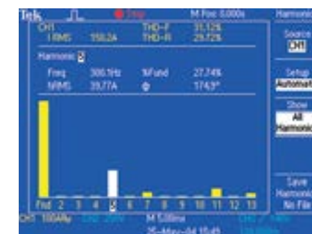
Conduct harmonic distortion measurements with TPS2PWR1 power measurement software.
