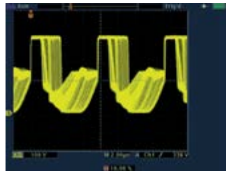
High waveform capture rate combined with intensity grading reveals modulation effects on a power supply control loop.
